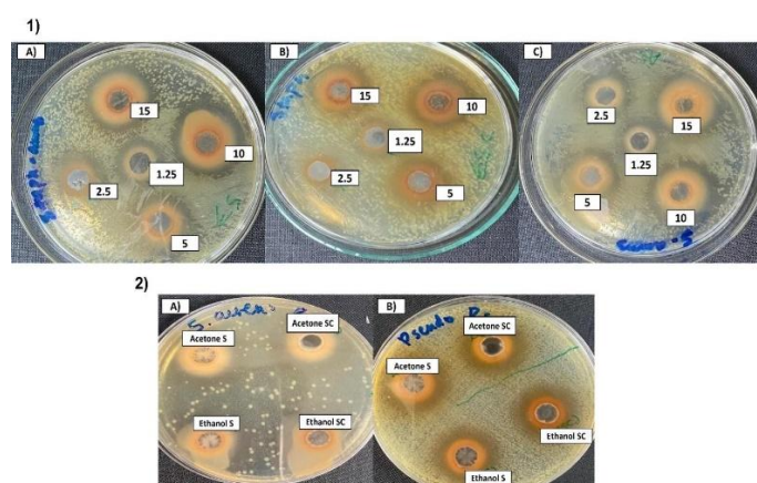
Figure 1: Bacterial inhibition using well-diffusion method. 1) Secondary metabolites inhibition against S. aureus (Conc. 1.25 -15 mg/mL), A) ethanolic seed extract (cotyledon), B) ethanolic seed coat extract, and C) acetonetic seed extract (cotyledon). 2) seed cotyledon and seed coat of ethanolic and acetonetic extracts against resistant bacterial strains (conc. 15 mg/mL). A) S. aureus R4 strain, and B) P. aeruginosa R5 strain.
