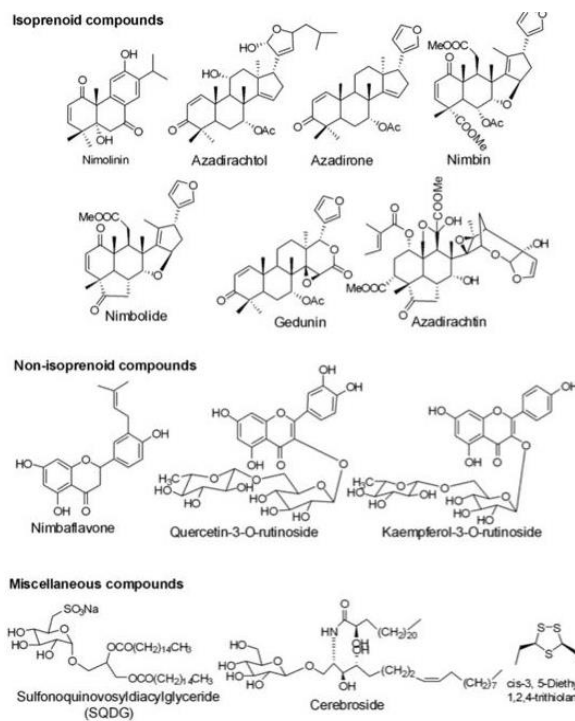
Figure 3: The major chemical compounds of neem leaf. [The name and structure of various compounds were described in the table above [10].
