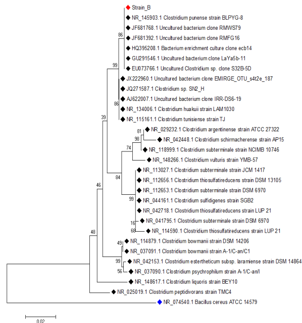
Figure 2: Dendrogram of Clostridium punense strain OFOb
