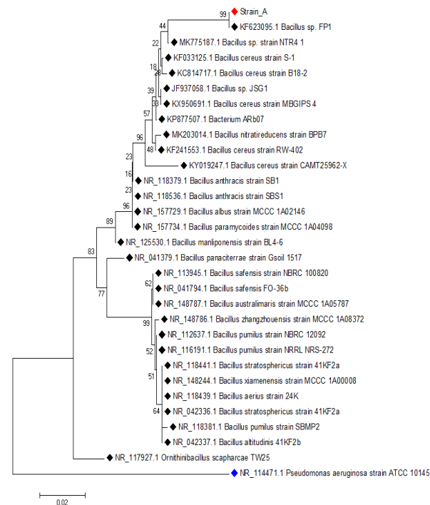
Figure 1: Dendrogram of Bacillus paramycoides strain OFO
