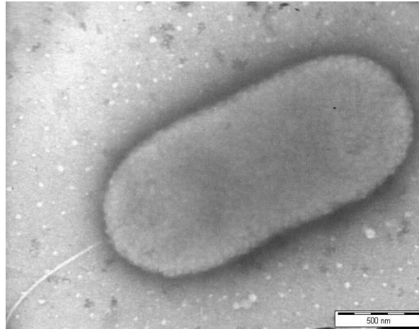
Figure 2A: TEM image of rod-shaped Klebsiella pneumoniae . (Magnification 28000x).
