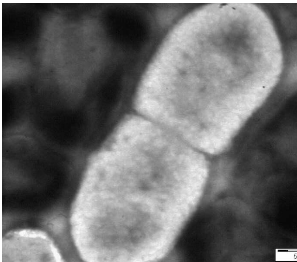
Figure 1B: TEM image show rod shaped bacteria with as in Klebsiella pneumoniae (Magnification 20000x)
