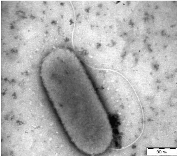
Figure 1A: TEM image of rod-shaped Klebsiella pneumoniae with a unipolar flagellar configuration (arrow). (Magnification 20000x).
