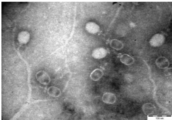
Figure 3B: EM image of Enterobacteria T6 phage (Magnification 106,000x).
