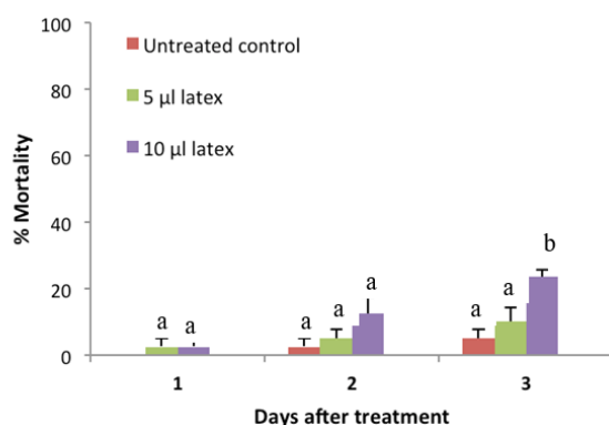
Figure 4: Mortality percentage (mean \pm SE) of S. littoralis larvae caused by different doses of latex serum. Bars with different letters were significantly different ( P < 0.05 ) by LSD after ANOVA.
