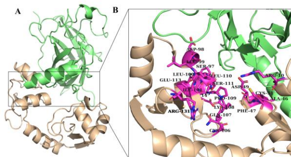
Figure 1: A) E6 and P53 protein complex B) The interface residues of E6 are shown in pink sticks interacting with the P53 (green).
