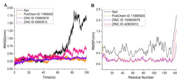
Figure 3: A) Demonstrates RMSD of Apo-E6 and three complexes plotted over the time of 100ns. A close analysis of the RMSD plot for all the systems clearly suggests that all the complexes were stable as compared to the Apo-E6. B) root mean square fluctuations (RMSF) of protein residues were plotted with respect to the residue number to show the local conformational changes for all the four simulations.
