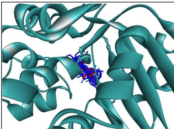
Figure 1: Visualization of the top ten compounds, as well as avibactam (red color), in the CTX-M-15 binding pocket.
