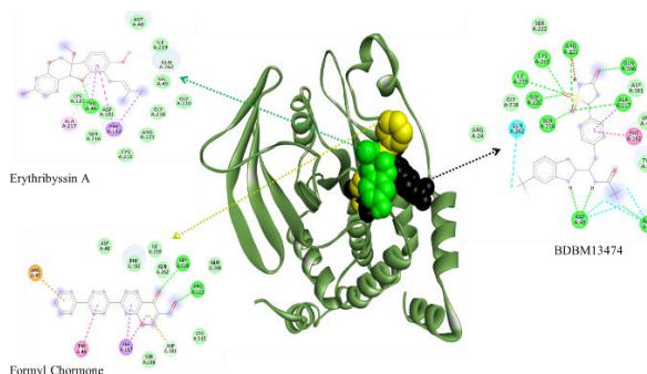
Figure 2: Binding poses and 2D interacting residues of PTP1B with control compounds.
