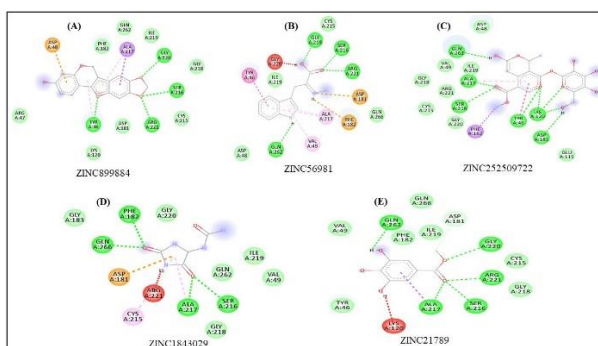
Figure 4: Interacting residues of PTP1B with ZINC899884 (A), ZINC56981 (B), ZINC252509722 (C), ZINC1843029 (D), and ZINC21789 (E).
