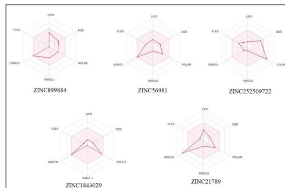
Figure 5: Bioavailability radar for top 5 hits (ZINC899884, ZINC56981, ZINC252509722, ZINC1843029, and ZINC21789).
