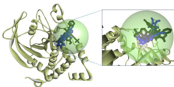
Figure 1: 3D visualization of docked poses of control compounds (black) and top 5 hits (blue) in the binding pocket of PTP1B.
