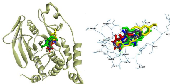
Figure 3: Binding poses of top 5 hits, ZINC899884 (green), ZINC56981 (grey), ZINC252509722 (yellow), ZINC1843029 (red), and ZINC21789 (blue) in the binding pocket of PTP1B.
