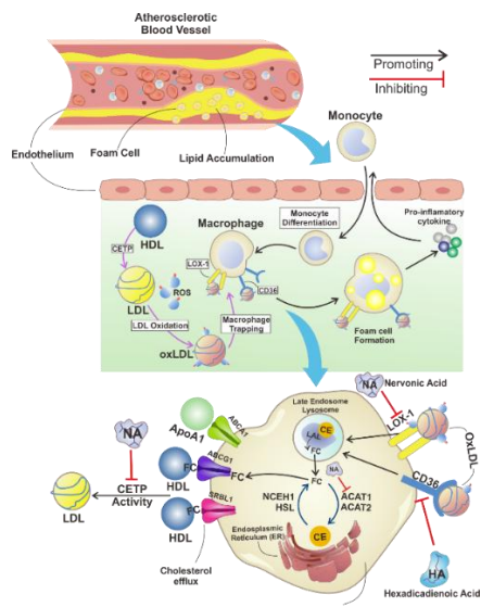
Figure 4: Schematic representation of the potential inhibitory effects of C. vulgaris 's fatty acids on foam cell formation. Cholesteryl ester transfer protein (CETP) facilitates the conversion of high-density lipoprotein (HDL) to low-density lipoprotein (LDL), leading to macrophage uptake and foam cell formation. Nervonic acid inhibits CETP activity, preventing HDL-to-LDL conversion. Additionally, Nervonic acid and Hexadecadienoic acid block lectin-like oxidized LDL receptor-1 (LOX-1) and CD36, reducing oxidized LDL (oxLDL) uptake by macrophages. The Nervonic acid also inhibits acyl-CoA:
