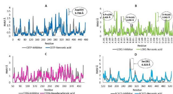
Figure 3: Molecular dynamic simulation results. (A) RMSF of CETP-ligand complex, (B) LOX1-ligand complex, (C) CD36-ligand complex, (D) ACAT1-ligand complex.
