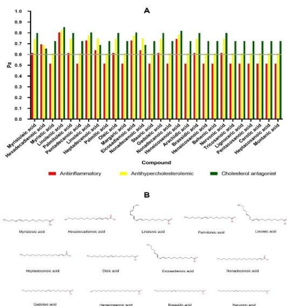
Figure 1: (A) Fatty acid bioactivity prediction with PASS online. (B) 2D structure of compounds that have anti-inflammatory, anti-hypercholesterolemic, and cholesterol antagonist activities.
