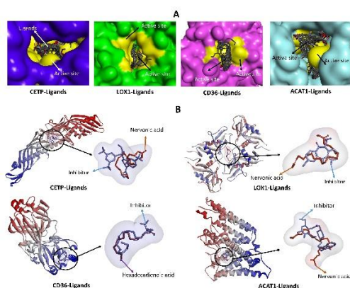
Figure 2: The molecular docking result between protein and ligand. (A) Protein docking results with all fatty acid and inhibitors. Yellow region represents an active site of the protein. Stick structure represents the fatty acid and inhibitors. (B) The visualization of the best molecular docking result of each protein.
