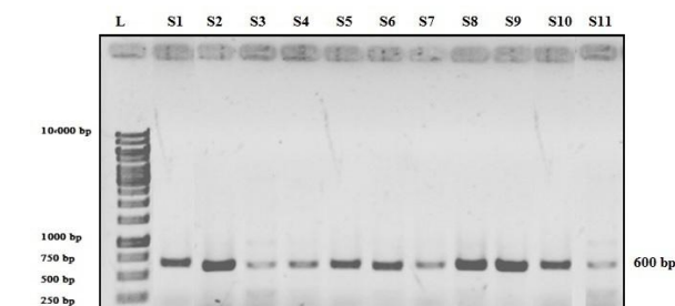
Figure 2: Amplification of strains with ITS (1 & 4) primers. All the eleven strains showing the position of PCR product near 600 bp, verifying the amplification for fungi.
